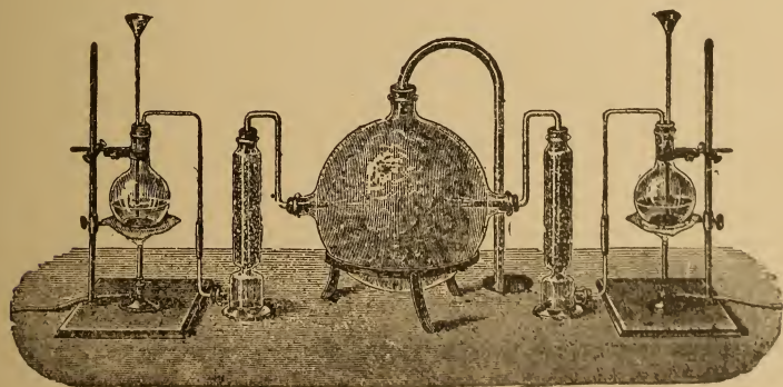
Fig. 98. APPARATUS FOR THE MANUFACTURE OF AMMONIA.
